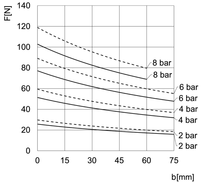
CGPT-20
