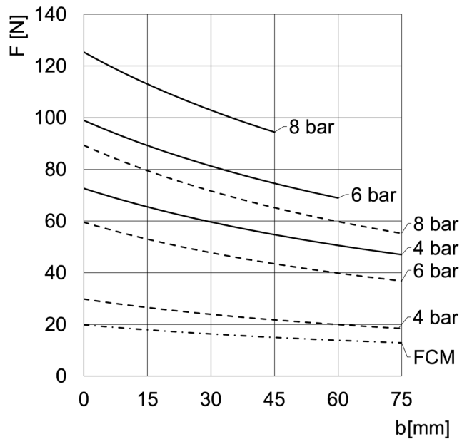
CGPT-20-NC
